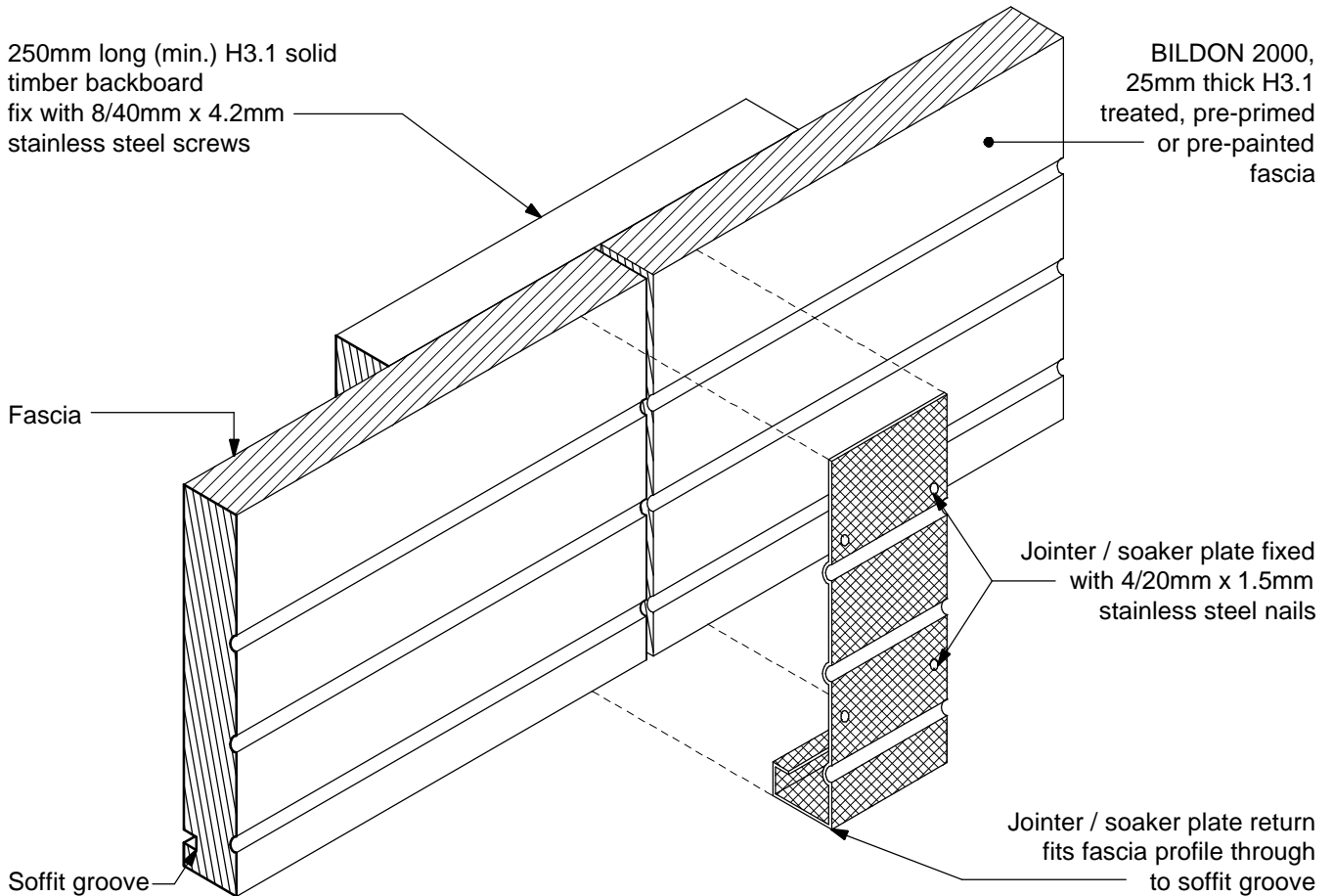
ISOMETRIC VIEW (soaker shown exploded)
