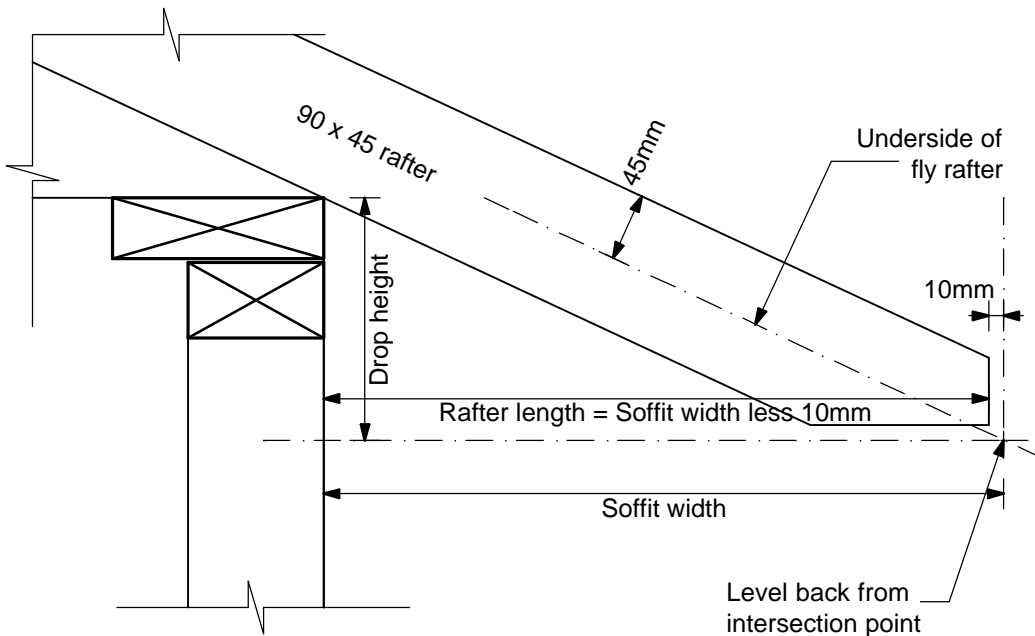
CONCRETE TILE ROOF SET OUT
