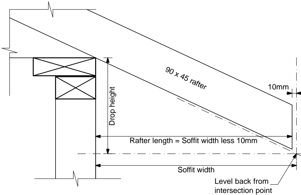
METAL ROOF SET OUT
