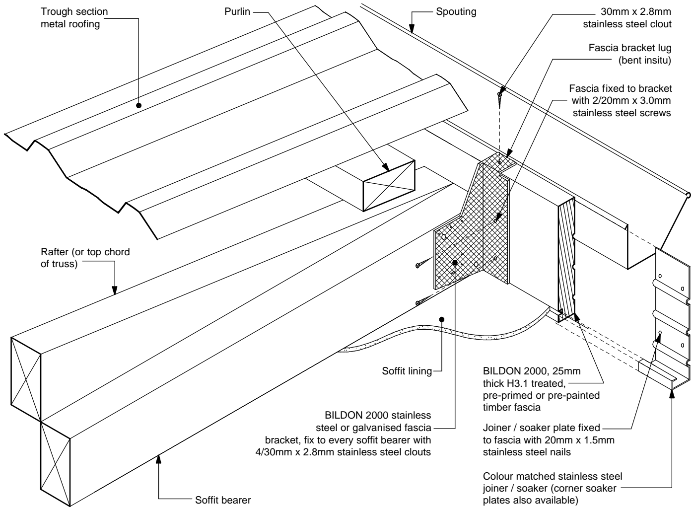
ISOMETRIC VIEW (soaker shown exploded)
